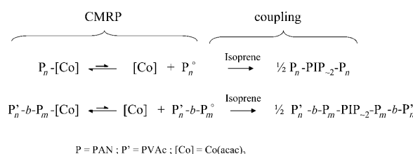
Scheme 1. General strategy for the coupling reaction of (co)polymers preformed by CMRP with isoprene. PAN = polyacrylonitrile, PVAc = poly(vinyl acetate), acac = acetylacetonato.
